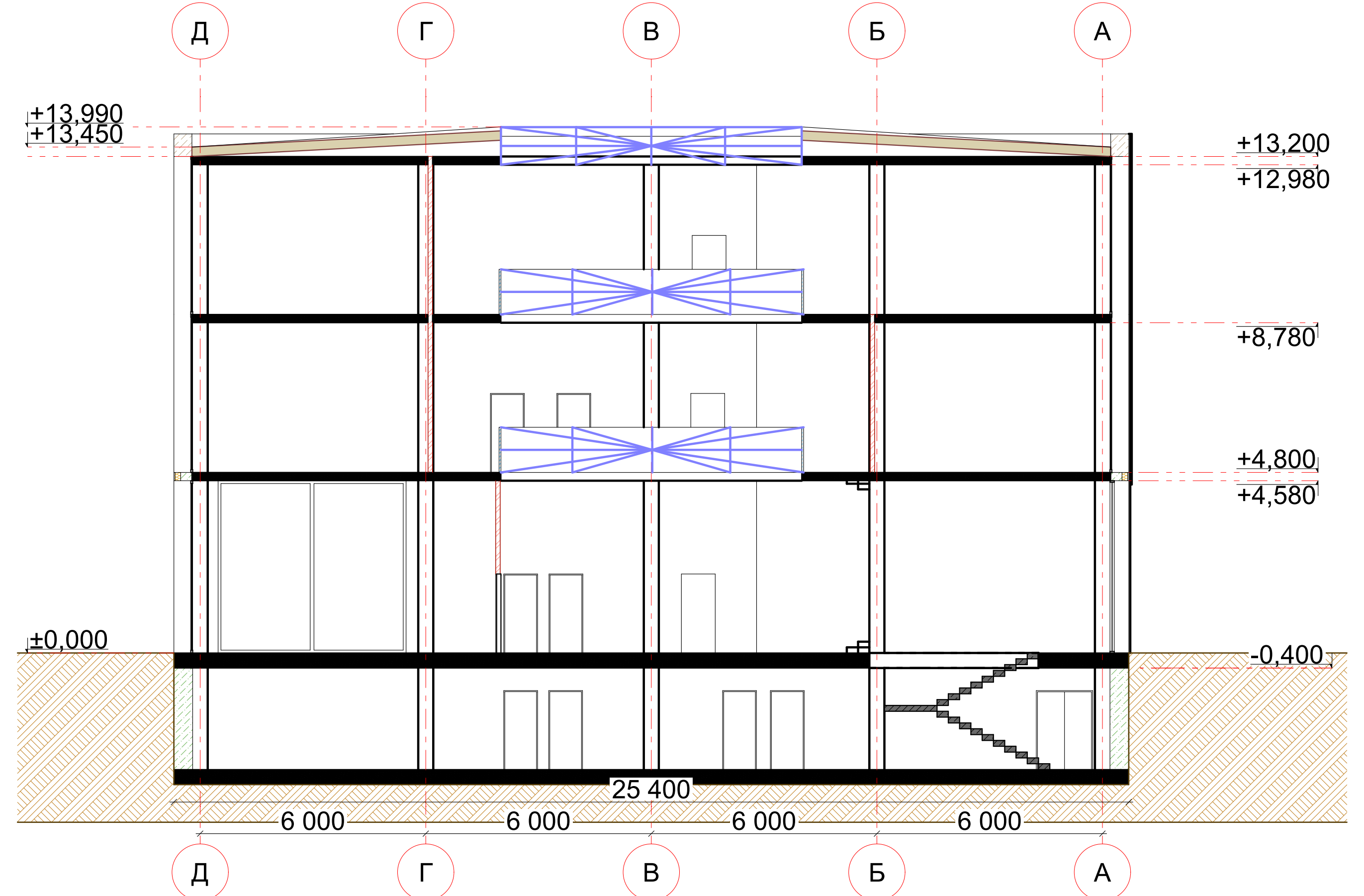
4-4 1:100
