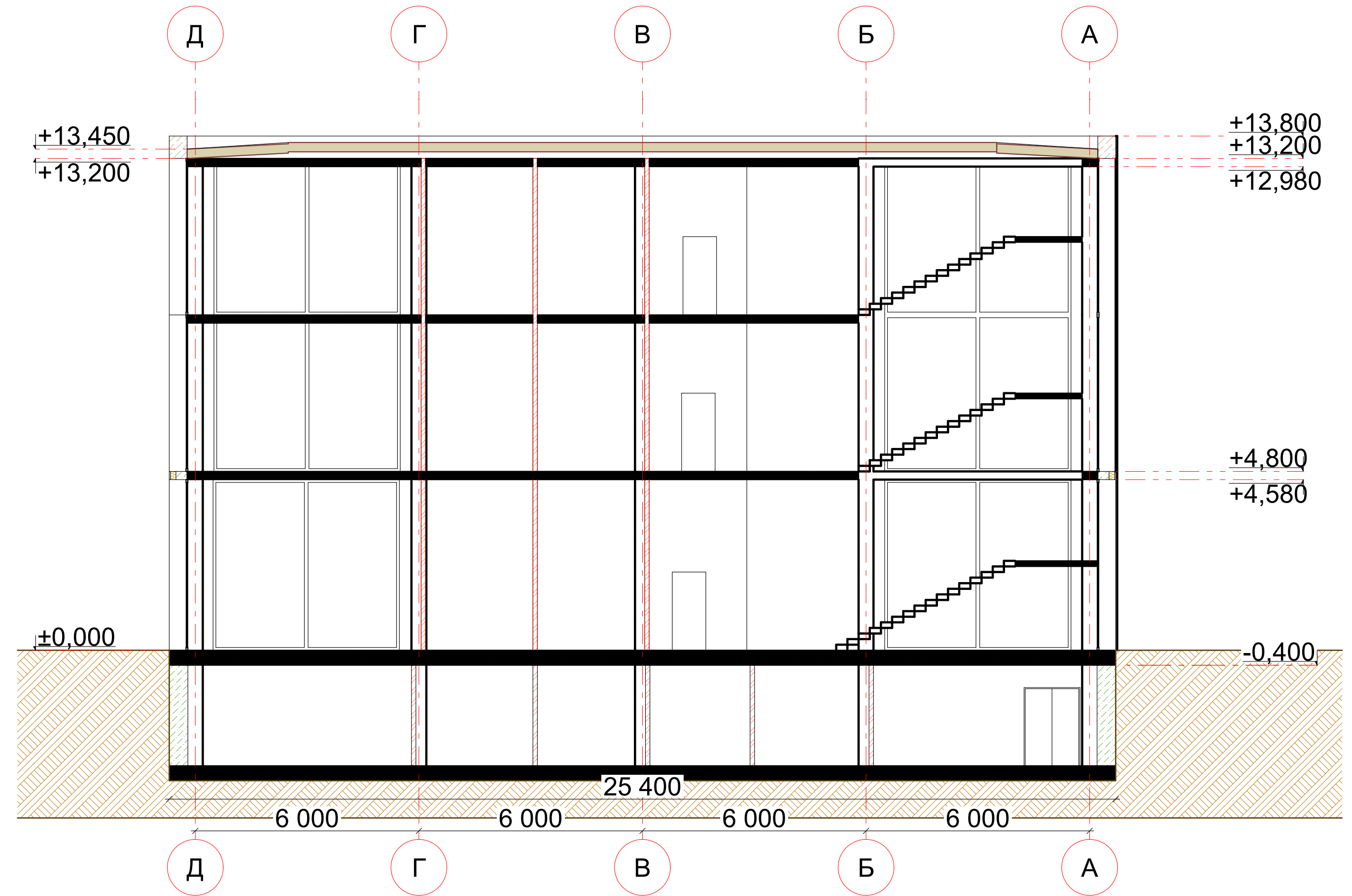
4-4 1:100
